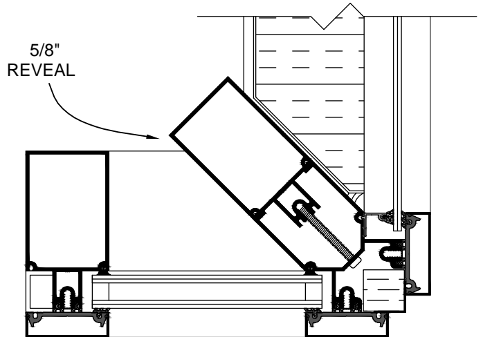
C2520 STANDARD CORNER
