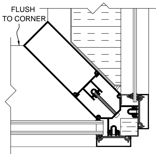
C2530 STANDARD CORNER
