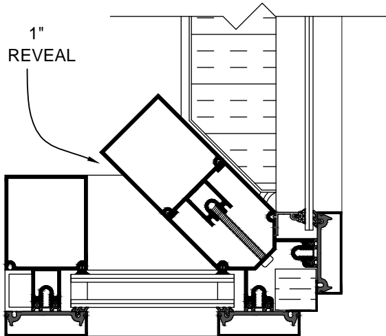
C2510 STANDARD CORNER
