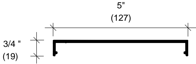
C2508 SNAP-ON CAP
