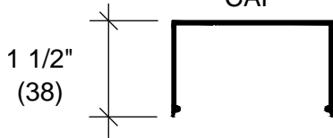
C2503 SNAP-ON CAP
