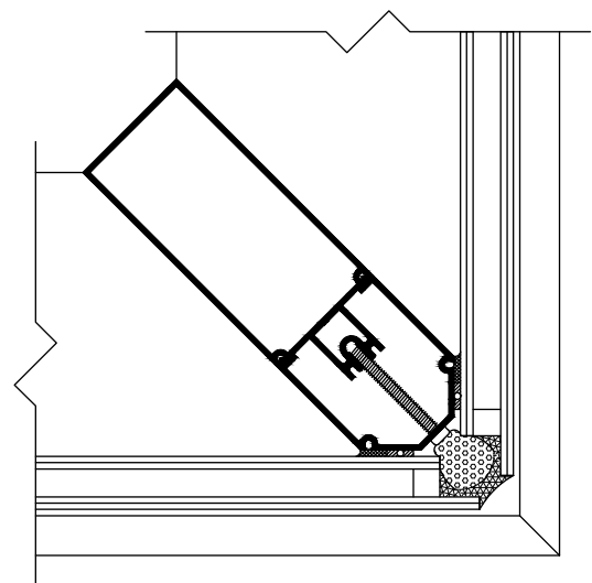
C2520 WITH NOSE REMOVED FOR SILICONE GLAZING
